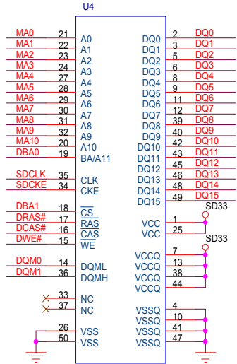
ESMT M12L16161A-7 NC
