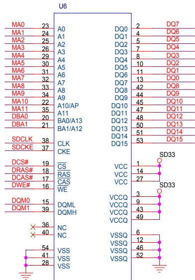
ESMT M12L64164A-7 TSOP54
