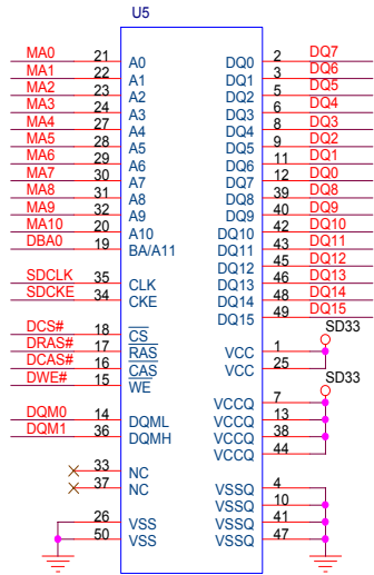
ESMT M12L16161A-7
